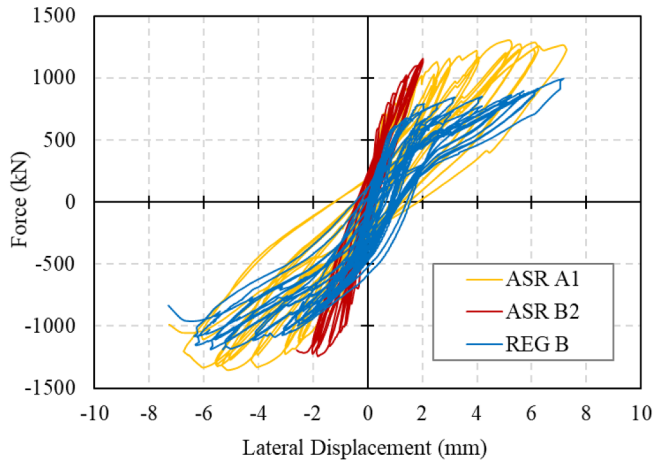
Fig. 4. Lateral load versus lateral displacement.
