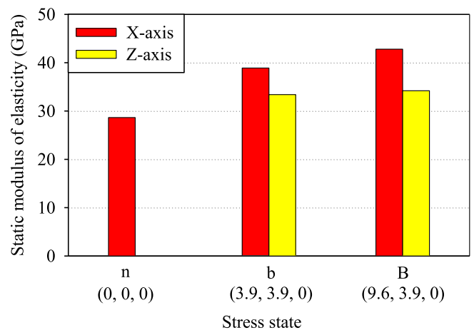
Fig. 2. Static modulus of elasticity along the stressed (X-axis) and unstressed (Z-axis) directions in the biaxially stressed specimens at 8 months of accelerated curing.
