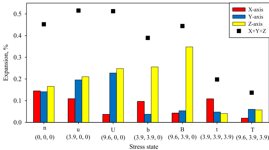
Fig. 1. Longitudinal and volumetric expansion (X+Y+Z) at 12 months of accelerated curing.
