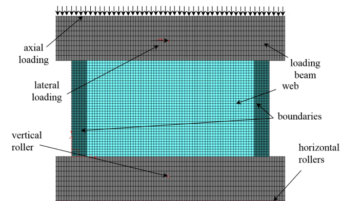
Fig. 6. Typical finite element model.
