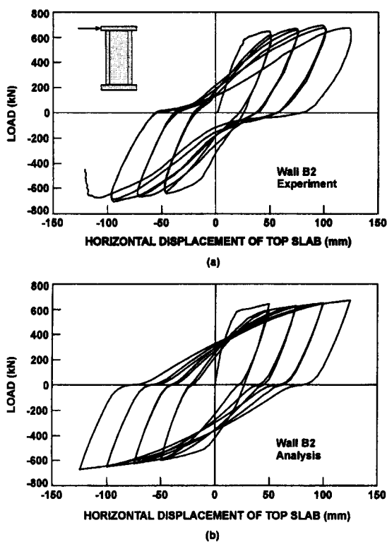
Fig. 3—Load-deformation responses of B2: (a) observed, taken from Oesterle et al., 13 and (b) calculated.
