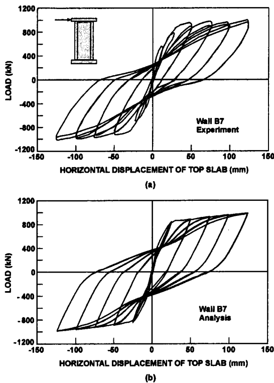
Fig. 4—Load-deformation responses of B7: (a) observed, taken from Oesterle et al., 13 and (b) calculated.
