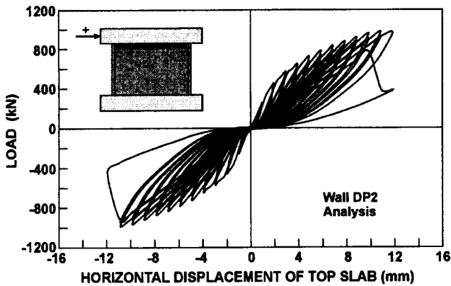
Fig. 16—Modified load-deformation response of DP2.
